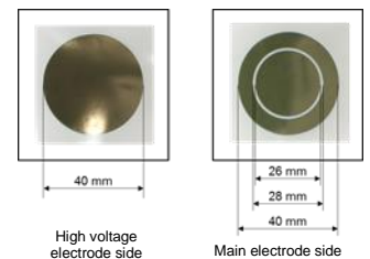
Fig. 2 Film's Geometry
