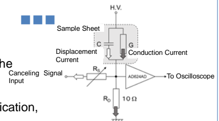
Fig.1 Detect Circuit
