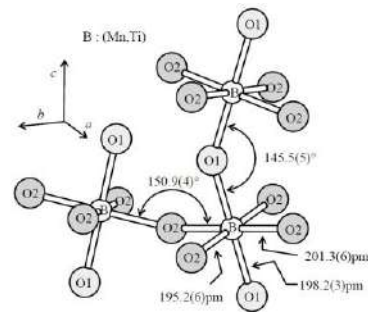
Distorted octahedron of \text{B}(\text{Mn}, \text{Ti}) ions.
