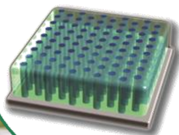
Micro-Phase Separation
